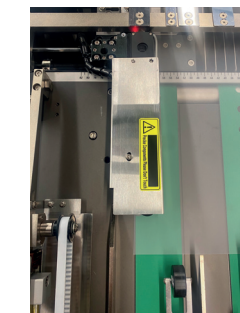
For initial screen register set-up, the camera is targeting the fiducial in the screen.
