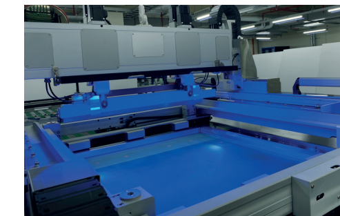
Blue LED light from top, camera from beneath checking the fiducial exposed in the screen.
