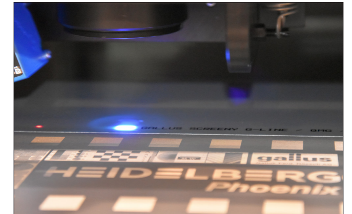
The automatic predictive autofocus is a highlight of the Phoenix CtS system. The autofocus system permanently measures the distance between the exposure head and the screen surface and automatically adjusts in the Z-direction for a constant depth of field during exposure for perfect quality.
