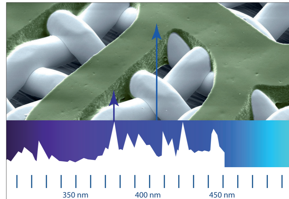
The 96 long-life lasers bundled into one beam expose at a wavelength of 405 nm for optimal crosslinking of the emulsions for perfect, reproducible quality.
